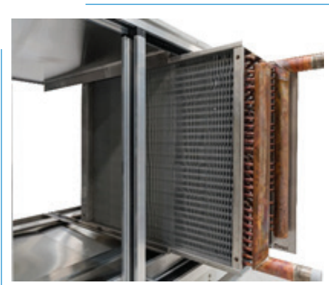
Fig 14: Coils Mounted on Slide Rail for Easy removal
